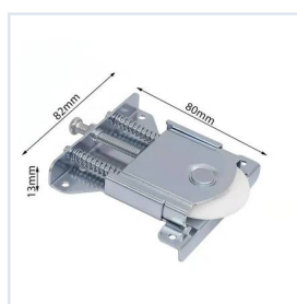
Sliding Door Roller Material: Iron+Plastic Surface: Zinc
