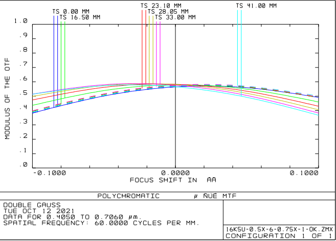
MTF VS Through Focus
