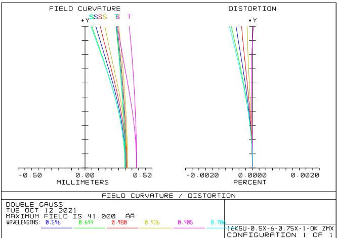
Distortion
