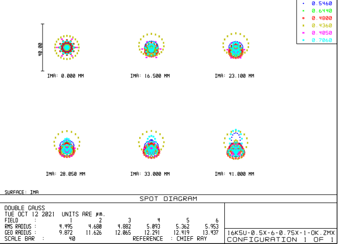
Spot Diagram
