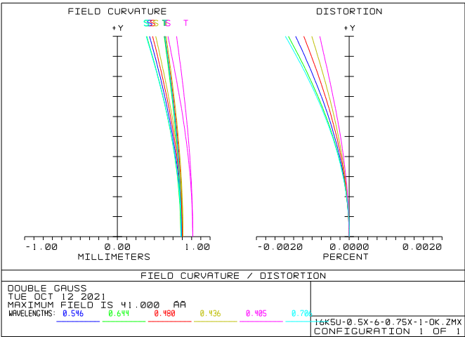
Distortion
