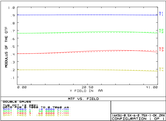
MTF VS Field 2.00X F4.0
