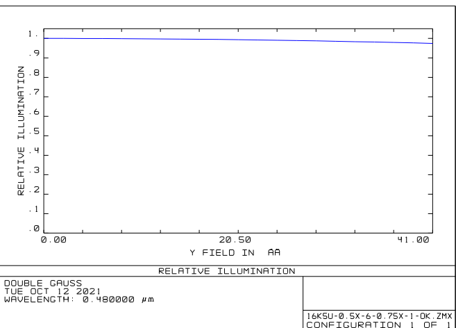
Relative Illumination
