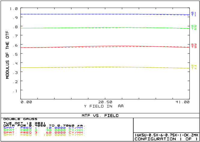
MTF VS Field 1.33X F4.0
