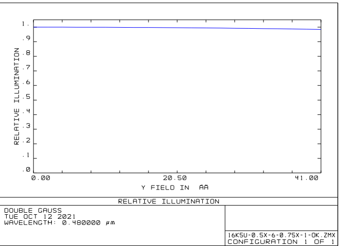
Relative Illumination
