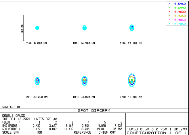
Spot Diagram
