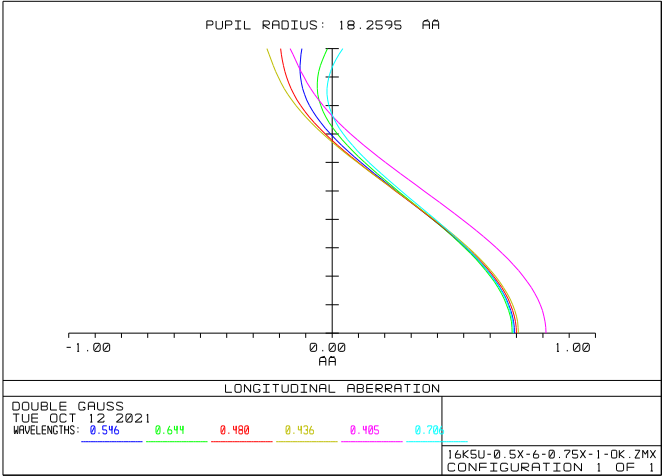
Axial color
