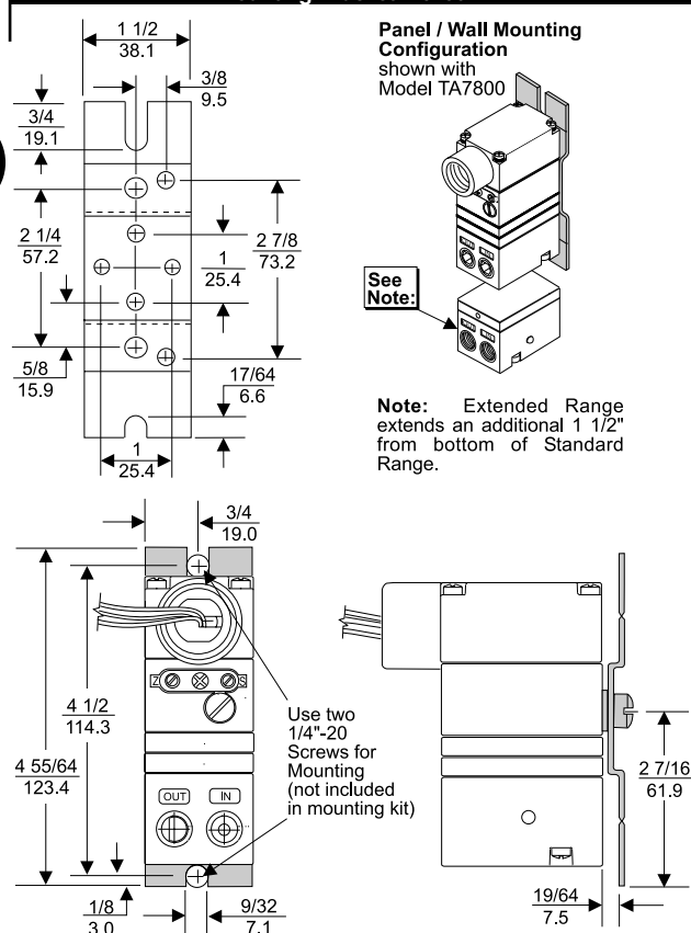
Mounting Bracket: 16893
