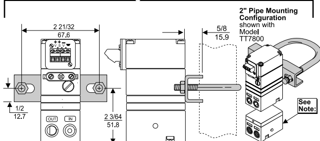
Mounting Bracket: 19254-1
