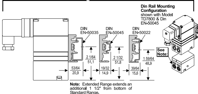
Mounting Bracket: 19254-1
