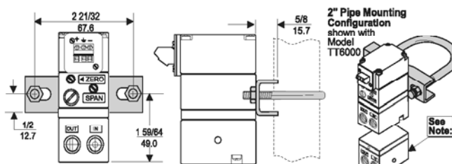
Mounting Bracket: 19254-1
