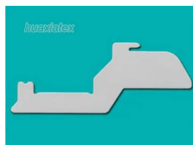
SINKERS Circular Knitting Machine Sinker PLTL-N04
