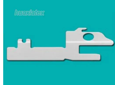
Circular Knitting Machine Sinker BX-22U
