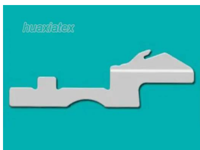
SINKERS Circular Knitting Machine Sinker PL-KS3BU-015
