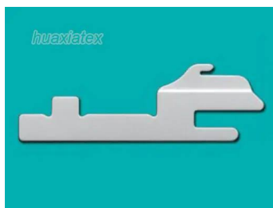
Circular Knitting Machine Sinker CF-22A5
