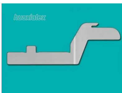
SINKERS Circular Knitting Machine Sinker P010-S05M
