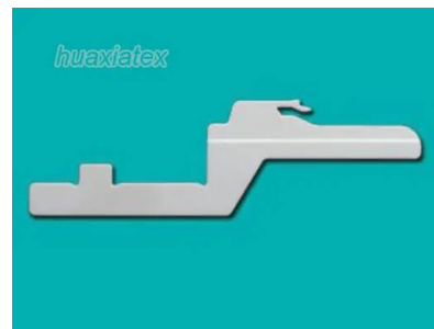
SINKERS Circular Knitting Machine Sinker PL-2.2U (LO OP2.2MM)
