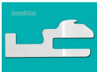
SINKERS Circular Knitting Machine Sinker GT-1305-LB
