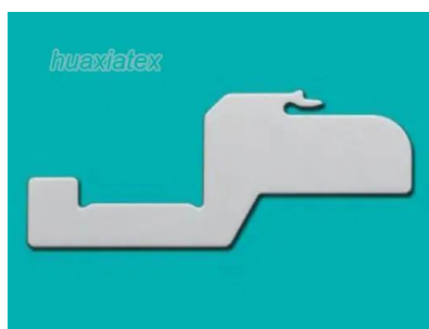
SINKERS Circular Knitting Machine Sinker 0001-TR01-2 .5 (LOOP2.5MM)
