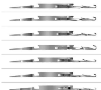
KNITTING NEEDLES Flat Knitting Needles
