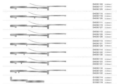
KNITTING NEEDLES Selectors for Sock Knitting Machines
