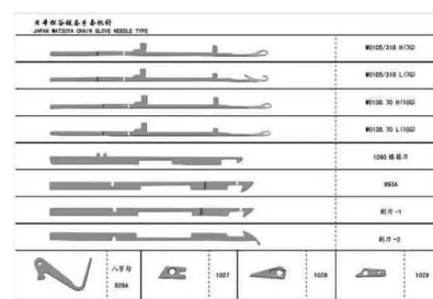
KNITTING NEEDLES Japan Matsuya Chain Glove Needle Type 7G, 10G
