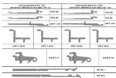
KNITTING NEEDLES Japan Matsuya Computerized Glove Needle Type 7G 10G
